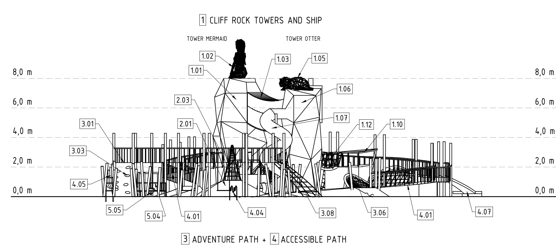
ELEVATION C1
