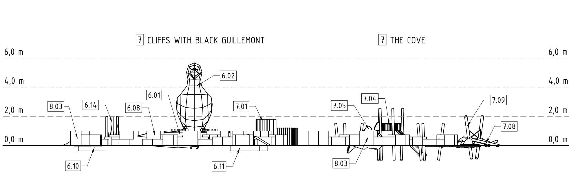
ELEVATION C2
